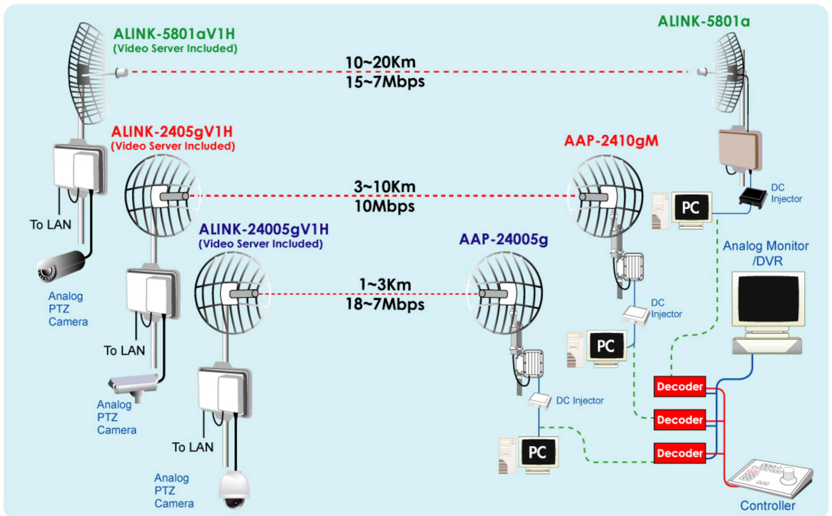
Point to Point Radio Link with Analog PTZ Camera, Transcoder and PC
